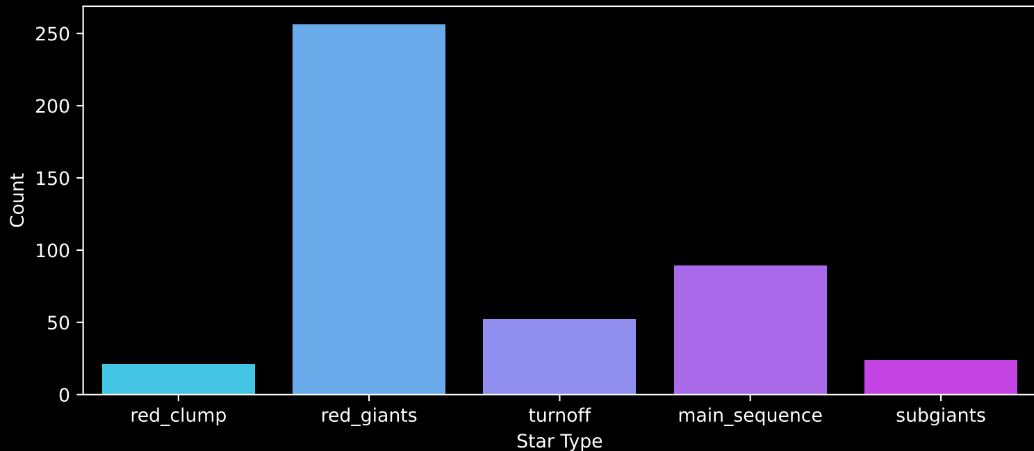
APOGEE DR17 Field: [N1333] Count plot of Star Type
