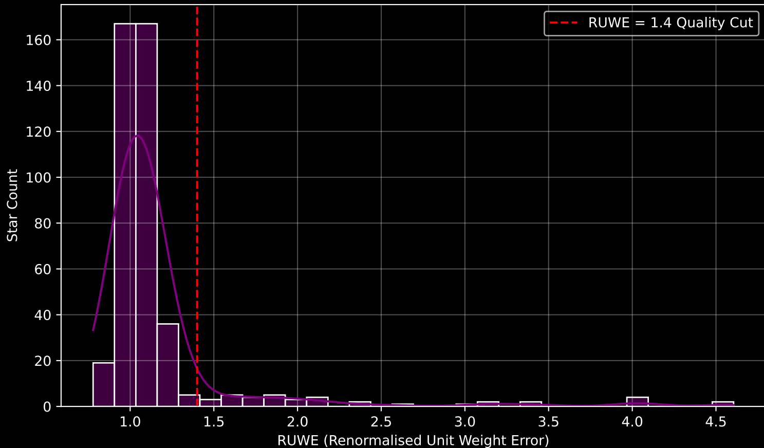
GAPOGEE DR17 Field [N1333] RUWE Distribution (n= 432)
