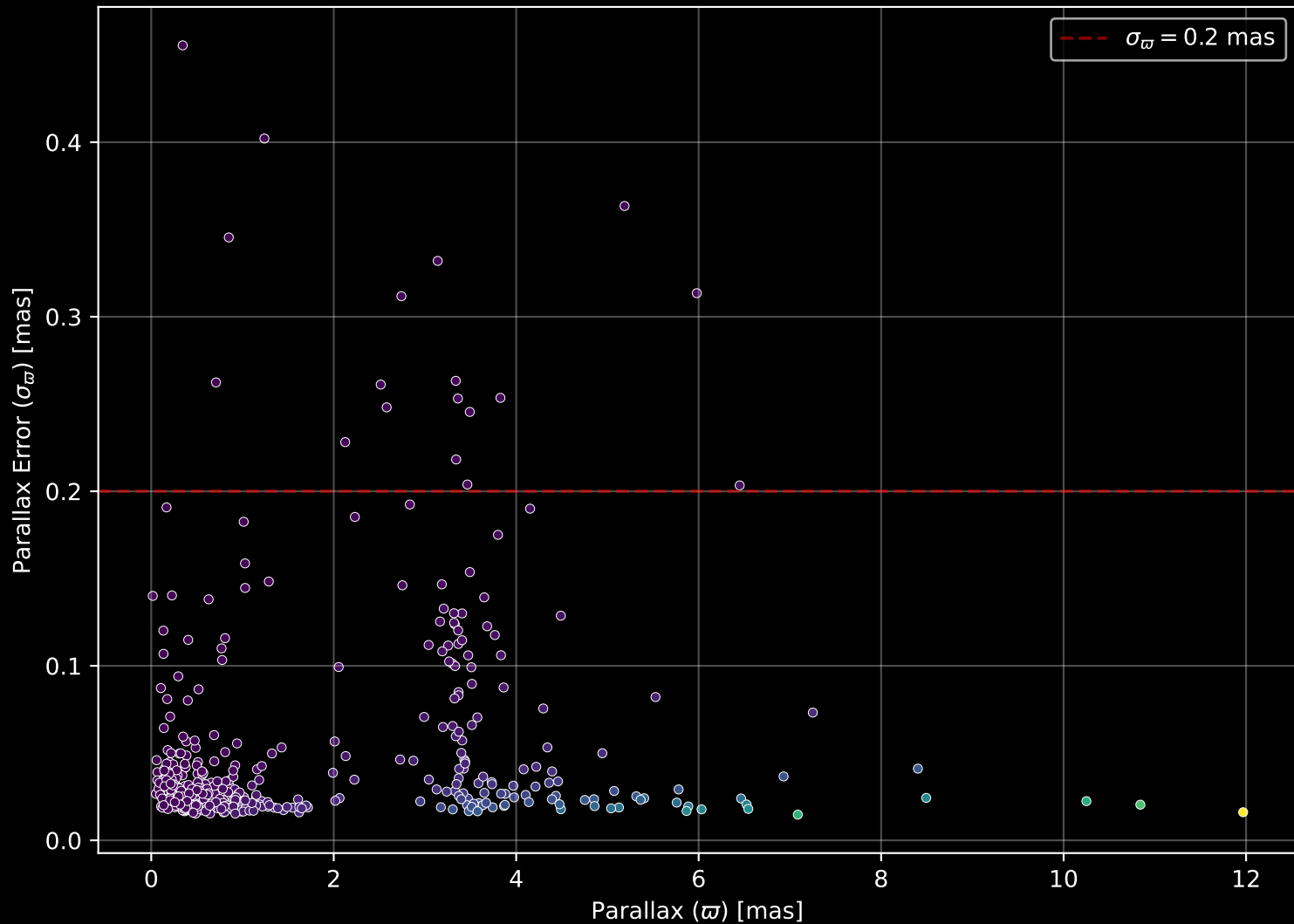
APOGEE DR17 Field: [N1333] Parallax Quality (n= 442)
