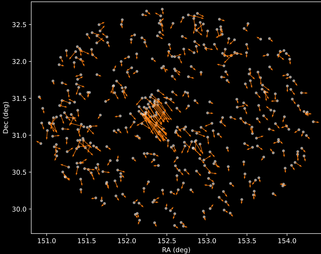
APOGEE DR17 Cluster 2 Proper Motion Vectors (n=412)
