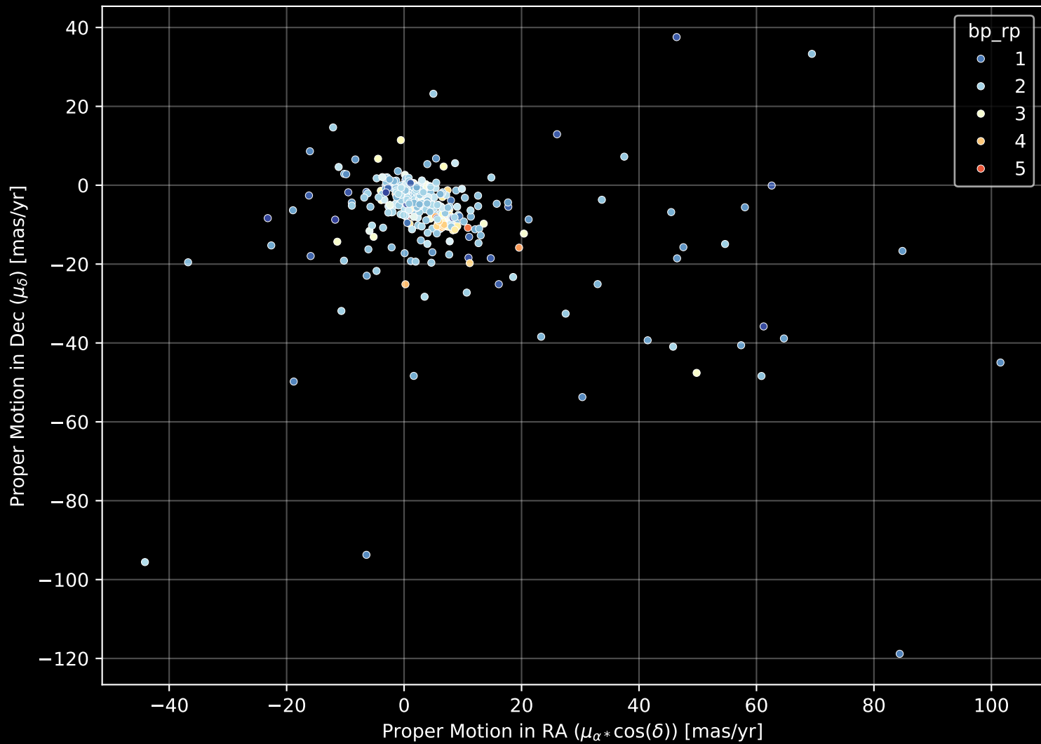
APOGEE DR17 Field: [N1333] Proper Motion Diagram (n= 442)
