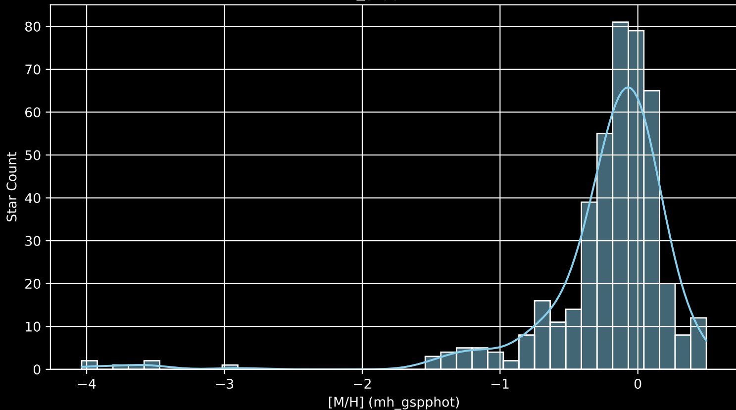
APOGEE DR17 Field: [N1333 [M/H] (mh_gspphot) (n= 438)
